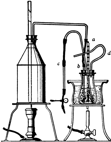
FIG. 156.—Apparatus arranged for the determination of the death-point of spores.
